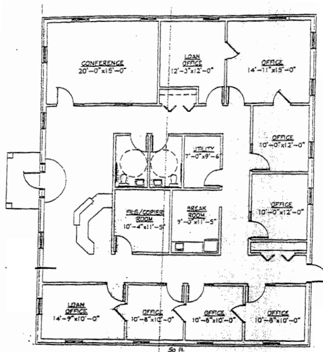
3,000 SF Office Floor Plan
